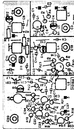
FRONTEND PCB
